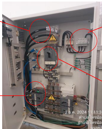
PV AC DB No.2 11SNB-WAC01
