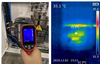
Breaker Inverter MCCB 35.6 °C
